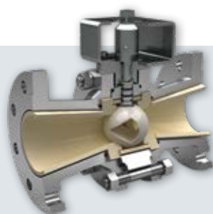
Ceramic-lined KST
