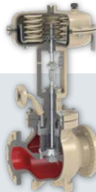
Steam Conditioning · 3281
